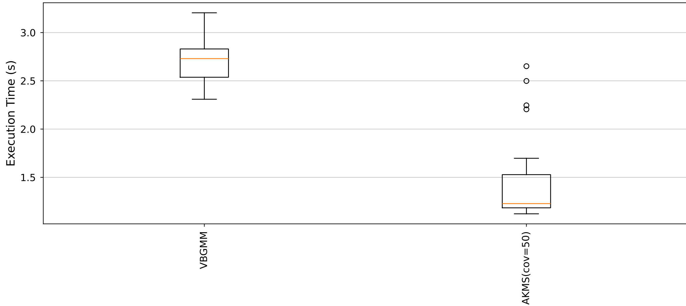
YARA Rules Execution Time Distribution (Cluster5_Size23 dataset)
